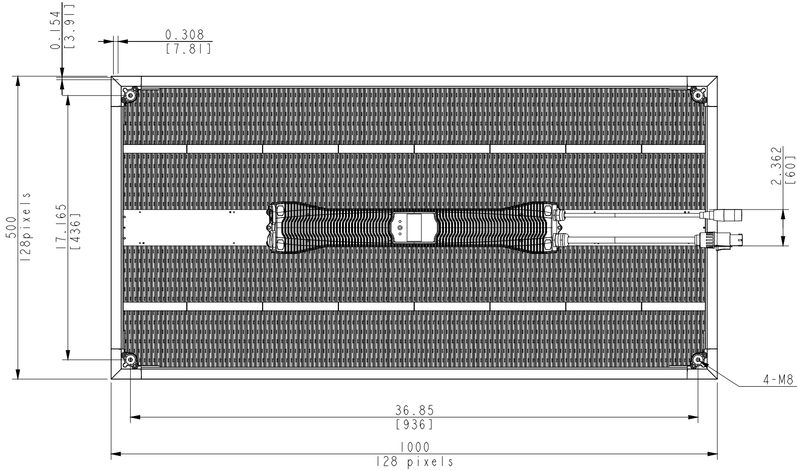
Rear View
